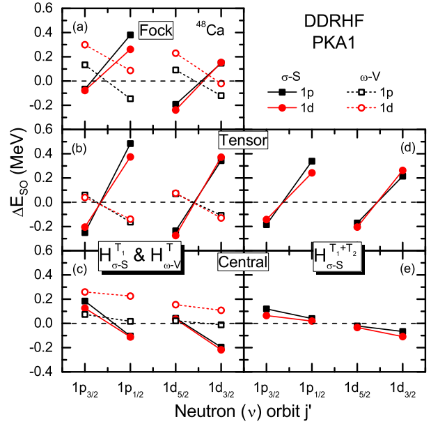
Fig. 1. (color online) Contributions to the spin-orbit (SO) splittings \Delta E_{SO} = V_{j_{-}j'} - V_{j_{+}j'} (MeV): the Fock terms [plot (a)], the tensor parts [plots (b) and (d)] and the central parts [plot (c) and (e)]. In plots (d-e), the supplemented tensor terms \mathcal{H}_{\sigma-S}^{T_2} are taken into account. The results are extracted from the calculations of DDRHF functional PKA1 for nodeless neutron ( \nu ) orbits in ^{48}\text{Ca} , and full Dirac spinors are utilized in calculating the interaction matrix element V_{jj'} .
