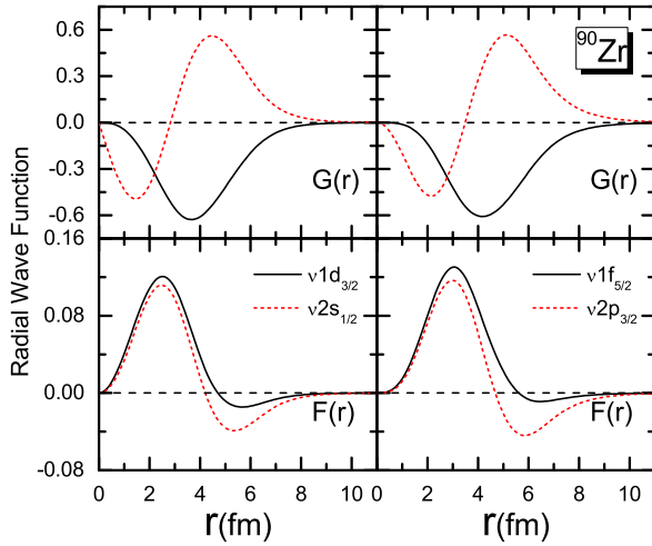
Fig. 3. (color online) Radial wave functions of the pseudo-spin partner states \nu 1\tilde{p} and \nu 1\tilde{d} in ^{90}\text{Zr} , where G(r) denotes the upper components and F(r) corresponds to the lower components. The results are extracted from the calculations of DDRHF with PKA1.
